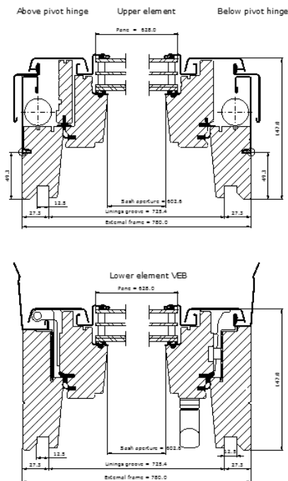
Horizontal section
